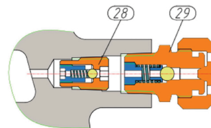
BODY GREASE FITTING SUB-ASSEMBLY DETAIL
